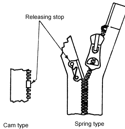
Figure 7 — Releasing stops
